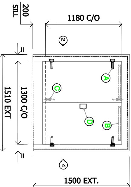
④ WALL 1 ELEVATION
