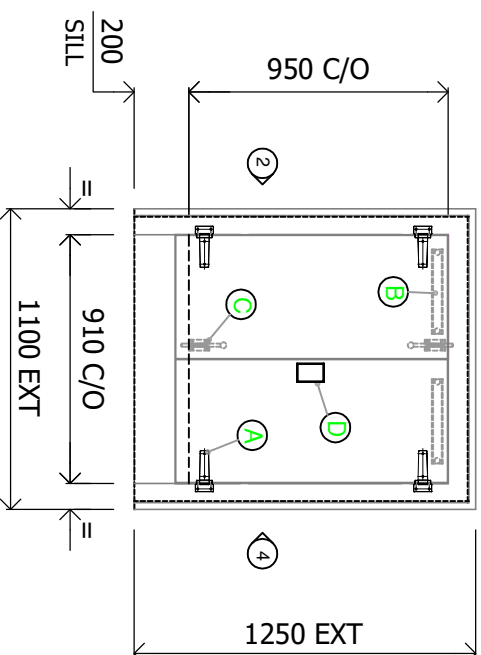
1 WALL 1 ELEVATION
